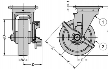
Drawing above shows the model with brake.
